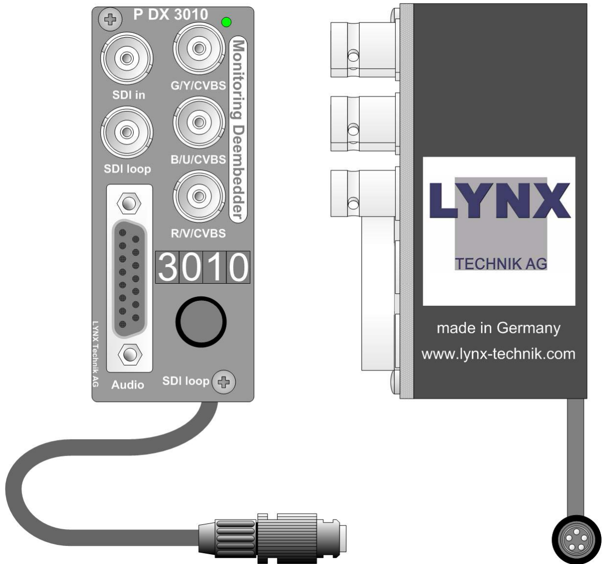
Figure 2 – Module Layout
