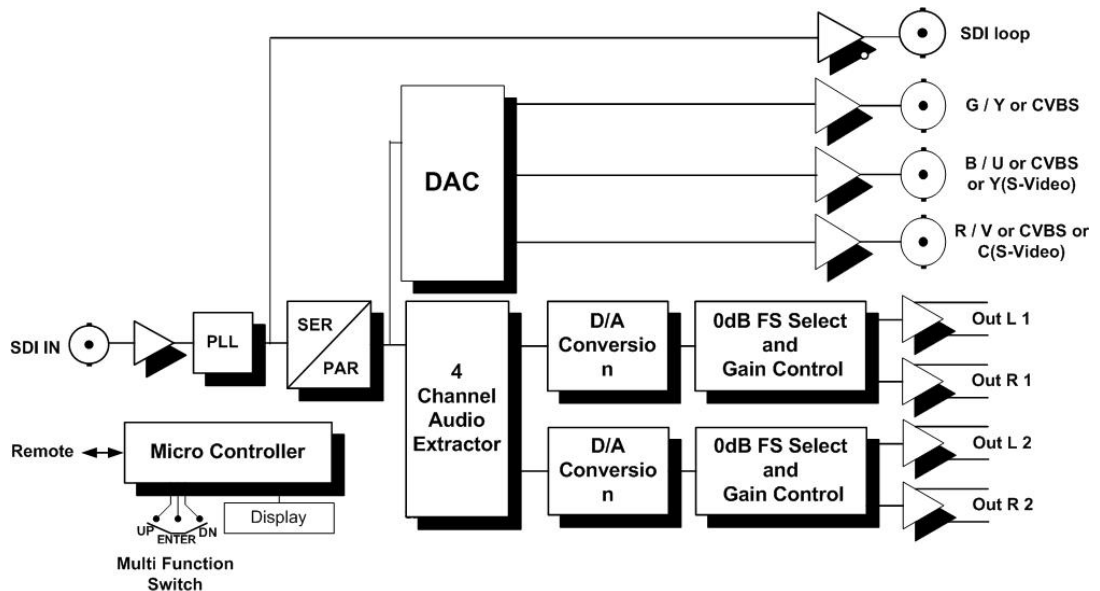
Figure 1- P DX 3010 Functional Diagram
